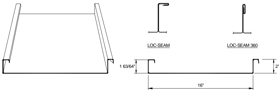
PANEL PROFILE
