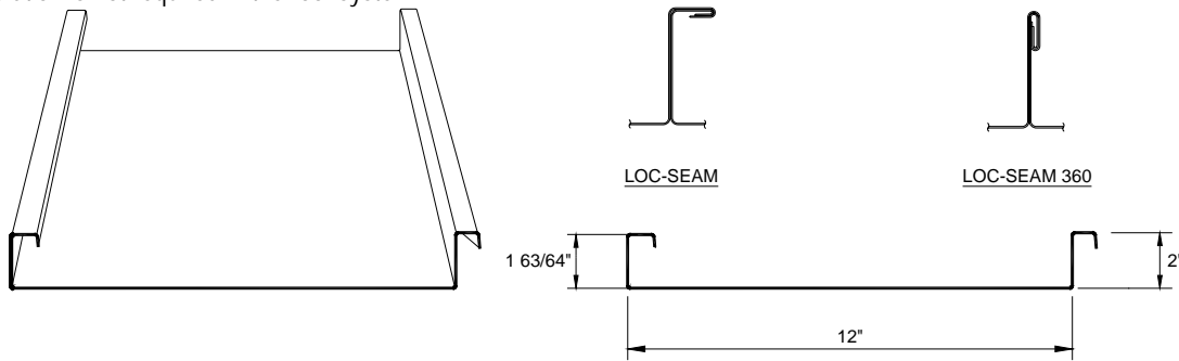
PANEL PROFILE
